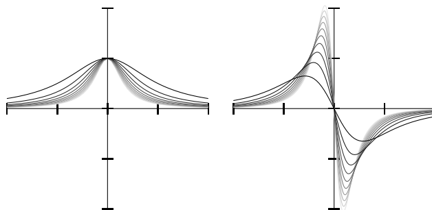
Figure 6.7: Graphs of \frac{1}{1+nx^2} and its derivatives for n = 1, 2, \dots, 10 , with higher n in lighter gray.
